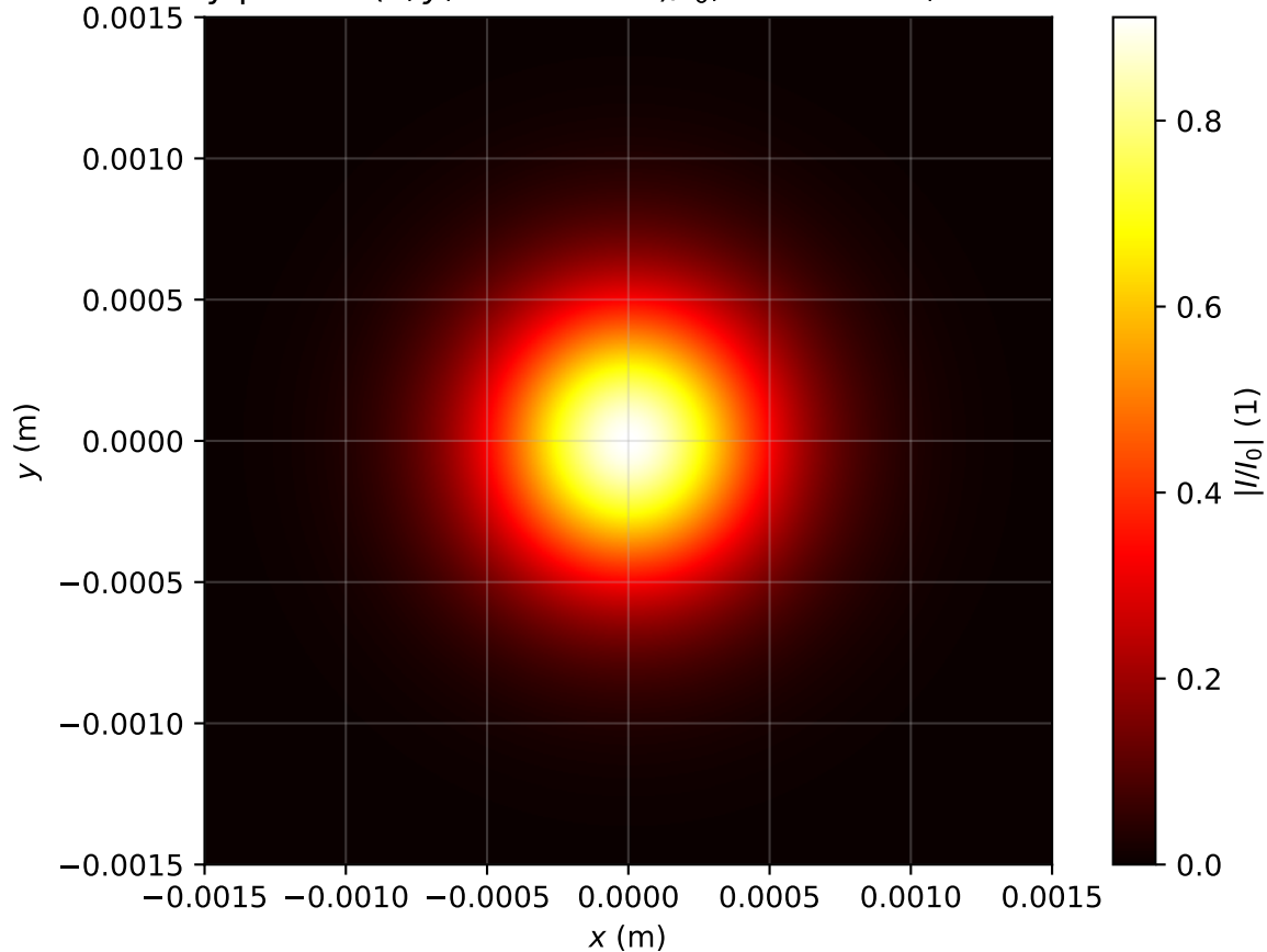
Intensity profile I(x, y, z = 1.353m)/I_0 , \text{Pin}=0.4\text{Pcr} , artificial time
